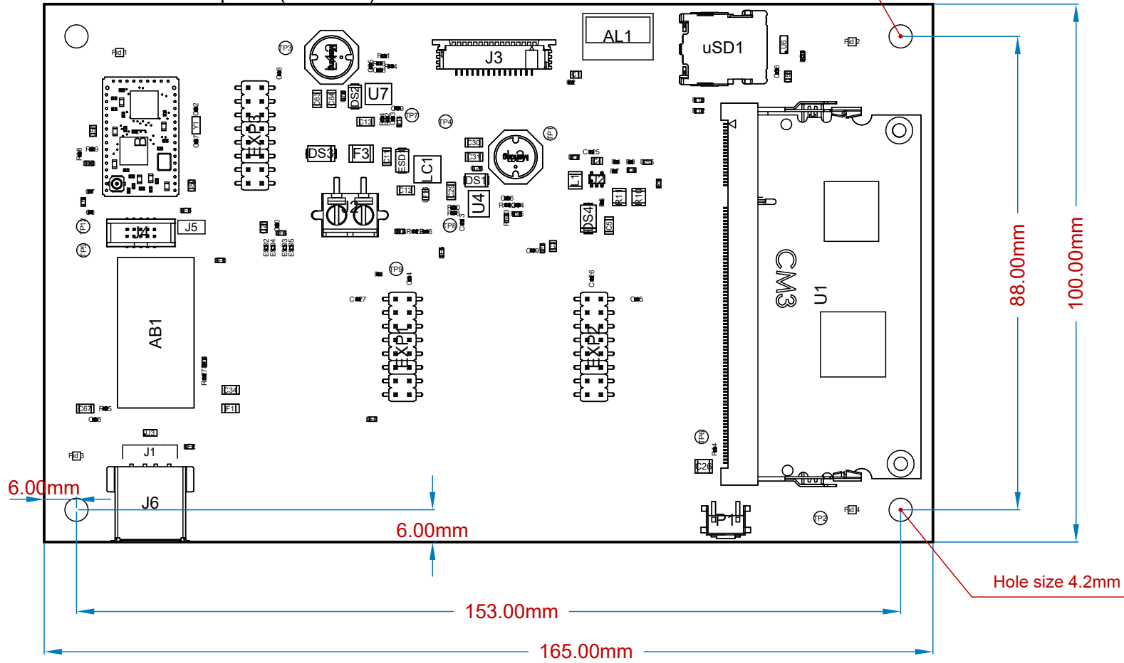
Board View from Top side (Scale 1:1)
