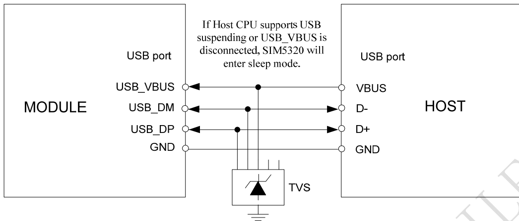
Figure 28: USB interface
