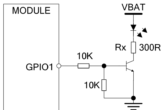
Figure 29: Application circuit
