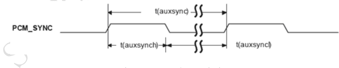
Figure 34: Synchrony timing
