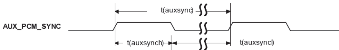
Figure 31: Synchrony timing
