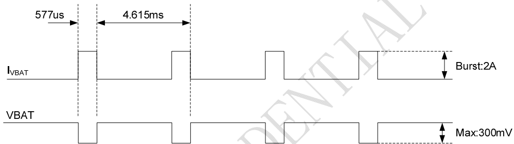
Figure 7: VBAT_RF voltage drop during burst emission (GSM/GPRS)
