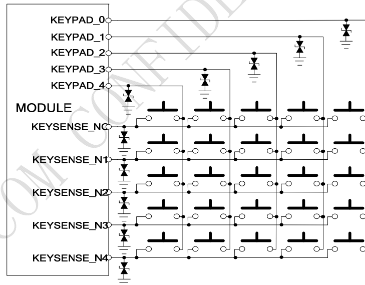
Figure 27: Reference circuit
