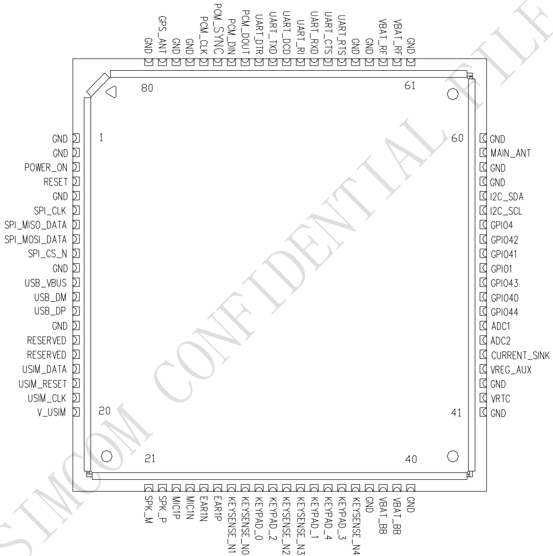
Figure 2: Pin view
