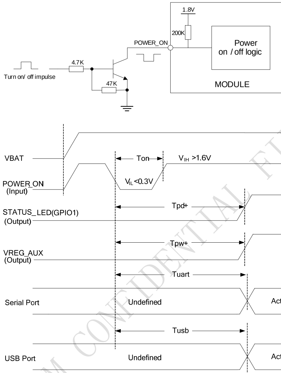
Figure 15: Power on Timing Sequence
