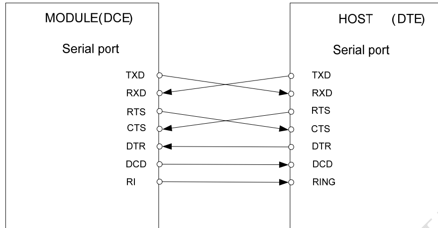
Figure 18: Full modem
