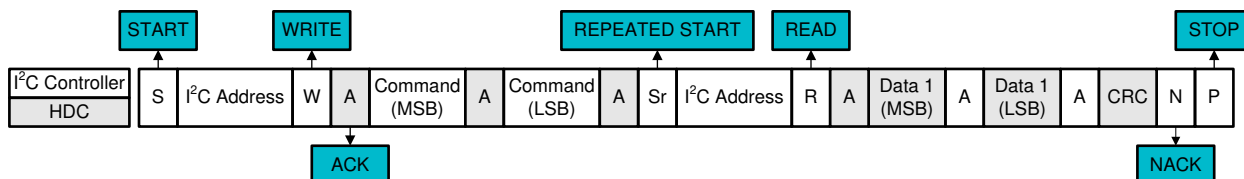
Figure 7-10. I 2 C Repeated START Sequence, Single Data Result, CRC Retained
