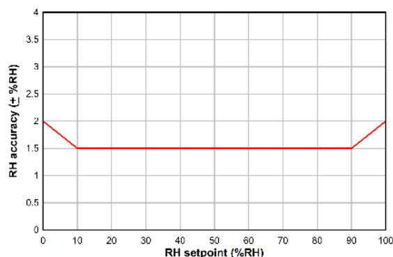
Typical RH Accuracy vs. RH Setpoint ( T_A = 25^{\circ}\text{C} )
