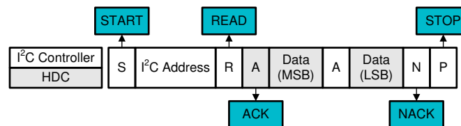
Figure 7-5. I 2 C Read Single Data Result, CRC Discarded
