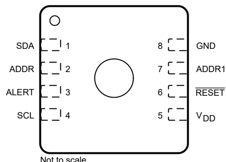
Figure 5-1. HDC302x DEF, DEH, or DEJ Package 8-Pin WSON Top View
