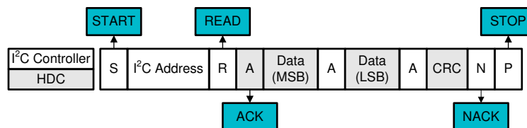
Figure 7-6. I 2 C Read Single Data Result, CRC Retained
